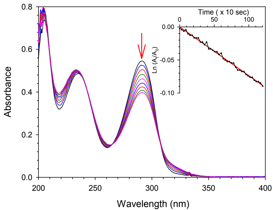
Fig. S1 UV-Vis absorption spectra of uric acid (0.05 mM in pH 6.8 phosphate buffer) over the course of the reaction with ^1\text{O}_2 . The insert shows the plot of \ln(A_t/A_0) as a function of reaction time, where A_t and A_0 are the absorbance at 291 nm at different times and time zero, respectively.
