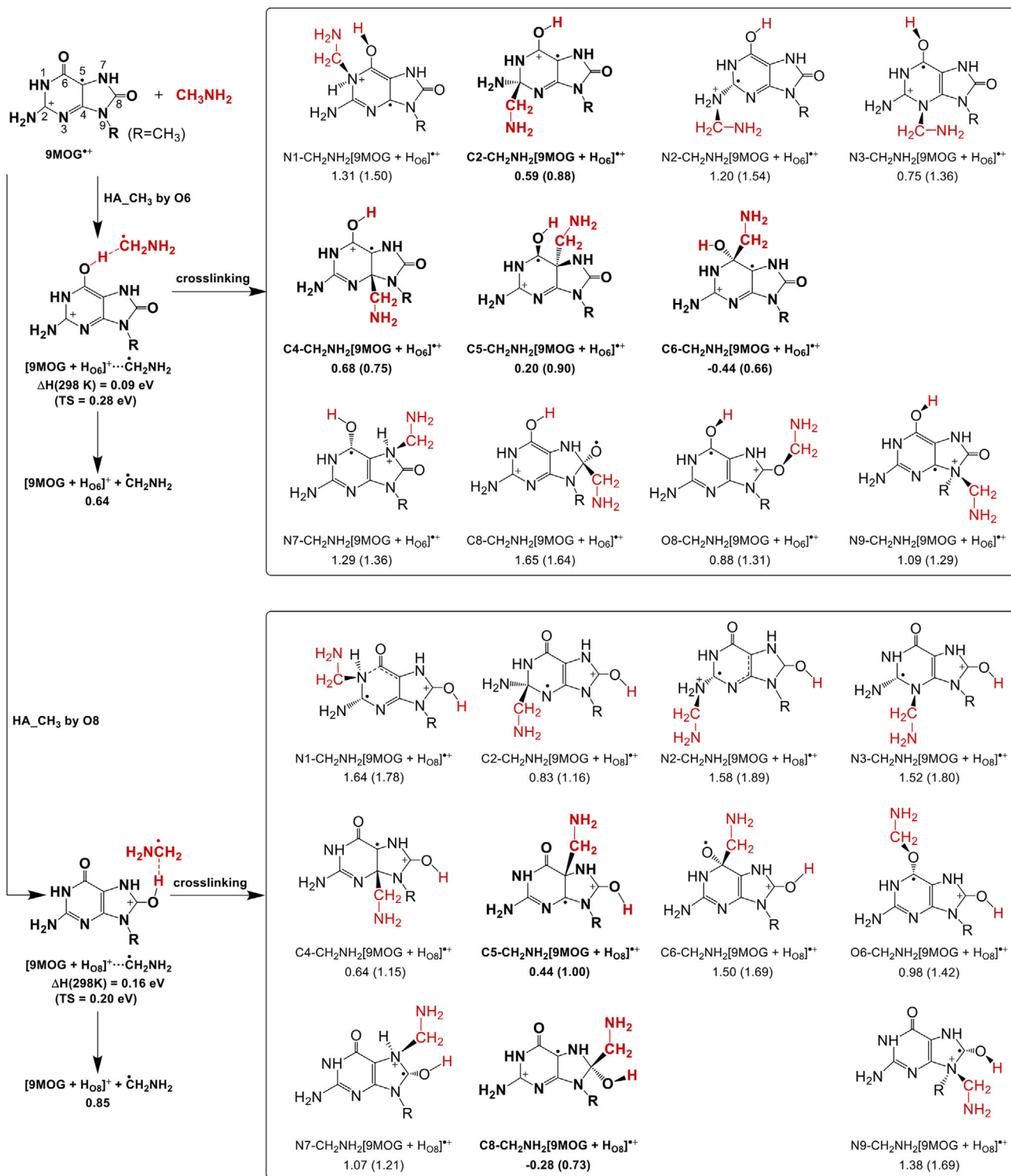
SCHEME 3 | Crosslinking following HA 3 by O6 and O8 of 9MOG + . Reaction \Delta H(298\text{ K}) and barriers (in parentheses) were calculated at DLPNO-CCSD(T)/aug-cc-pVQZ. Structures in bold represent probable high-energy crosslinks in the experiment.
