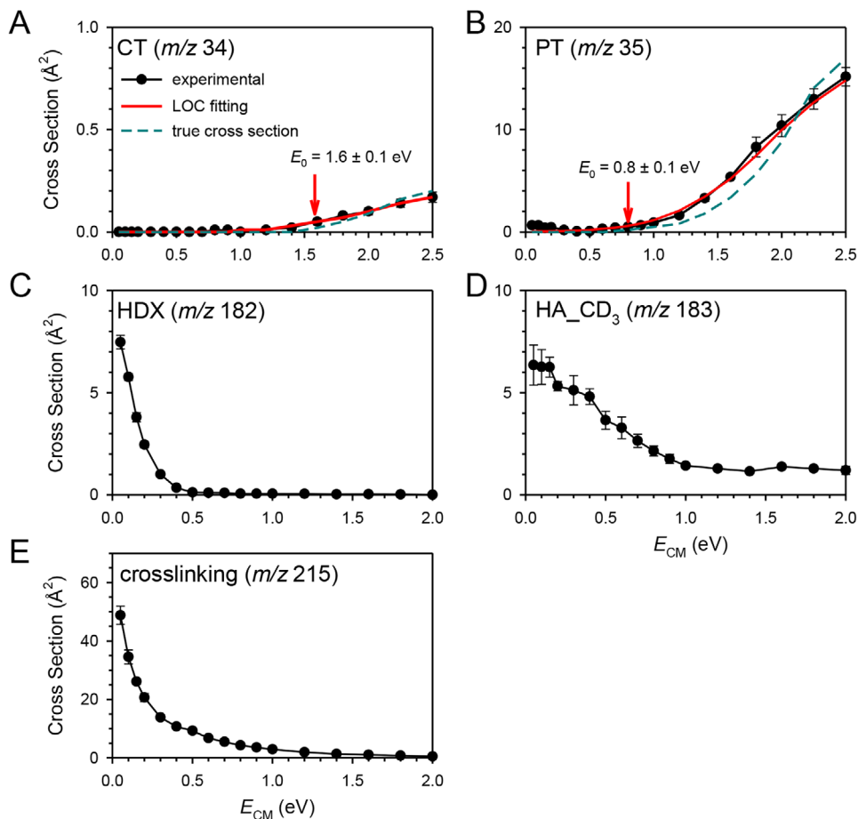
FIGURE 2 | Individual product cross sections vs. E_{\text{CM}} . Black plots represent experimental data, red curves show LOC fits, and cyan dashed lines denote true cross sections without energy broadening.
