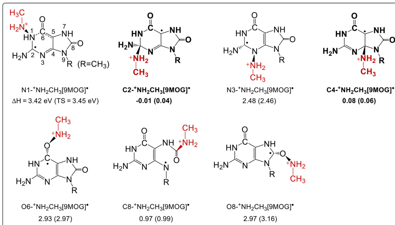
SCHEME 2 | Direct N -terminal addition of CH 3 NH 2 to 9MOG*+. Reaction Δ H (298K) and activation barriers (in parentheses) were computed at the DLPNO-CCSD(T)/aug-cc-pVQZ level. Structures in bold denote probable low-energy crosslinks in the experiment.
