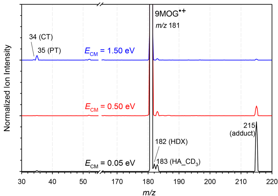
FIGURE 1 | Product-ion mass spectra for the reaction of 9MOG •+ with CD 3 NH 2 at E_{\text{CM}} = 0.05, 0.50, and 1.50 eV. Primary ion intensities were normalized to a unit for comparison.
